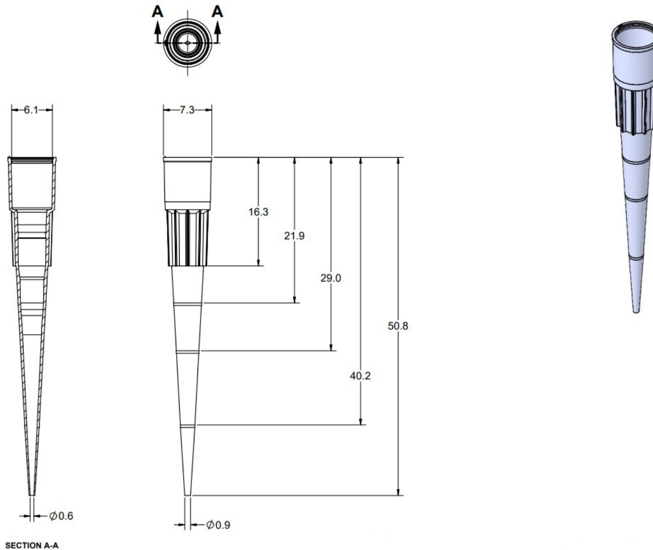
WB 6640 TripleA 200 ul LTS®-Compatible pipette tips Eco Refill, non-filtered
